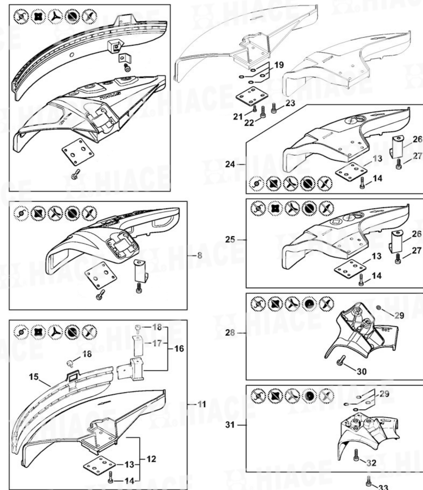
防護罩 Deflector
