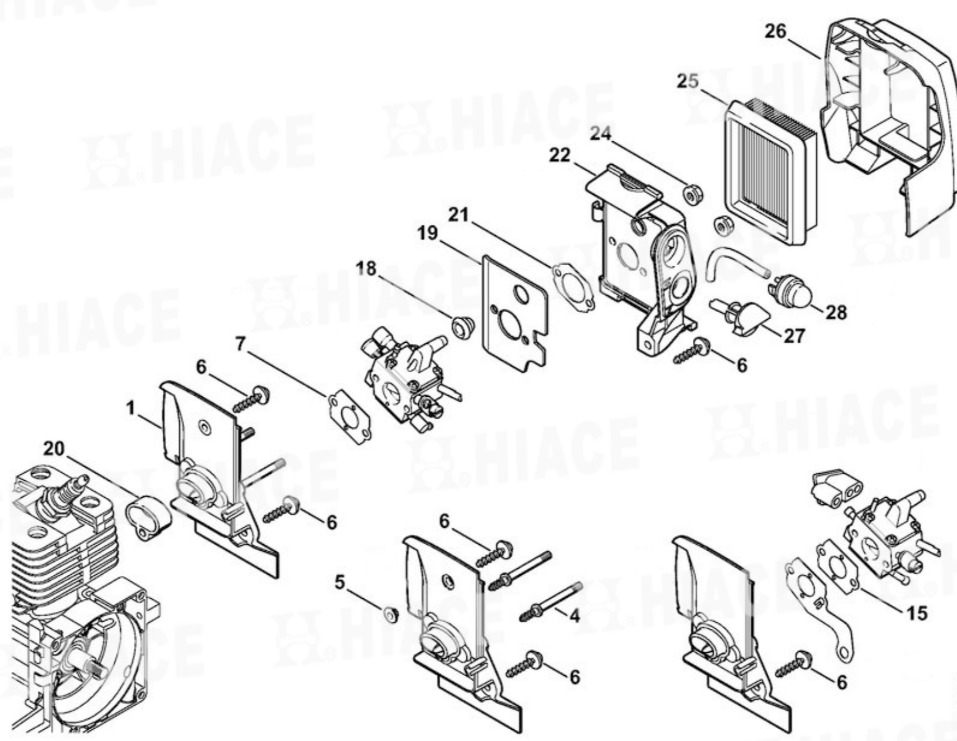
化油器外罩、空氣過濾器 Carburetor housing, Air filter 809 249 646
