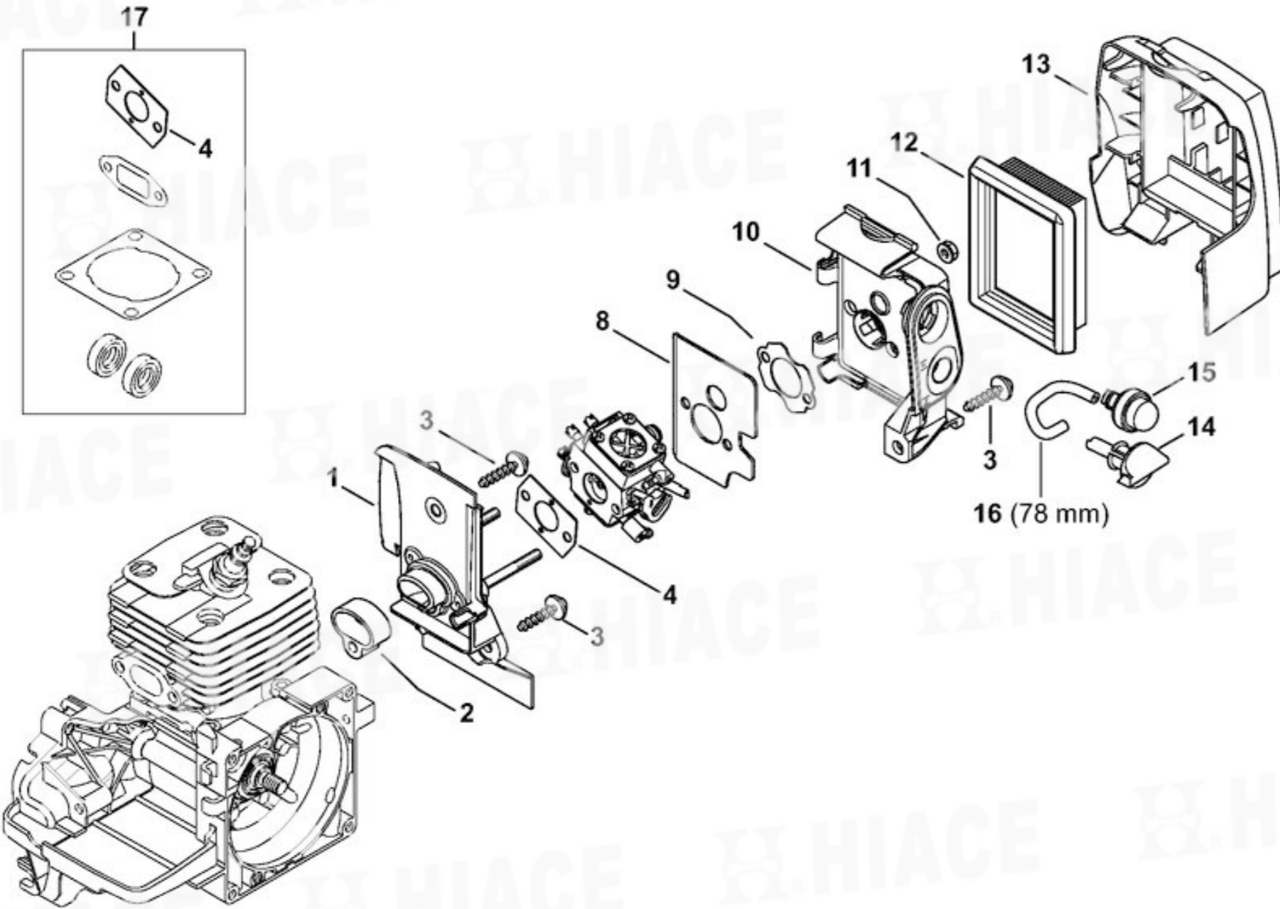
化油器外罩、空氣過濾器 Carburetor housing, Air filter
