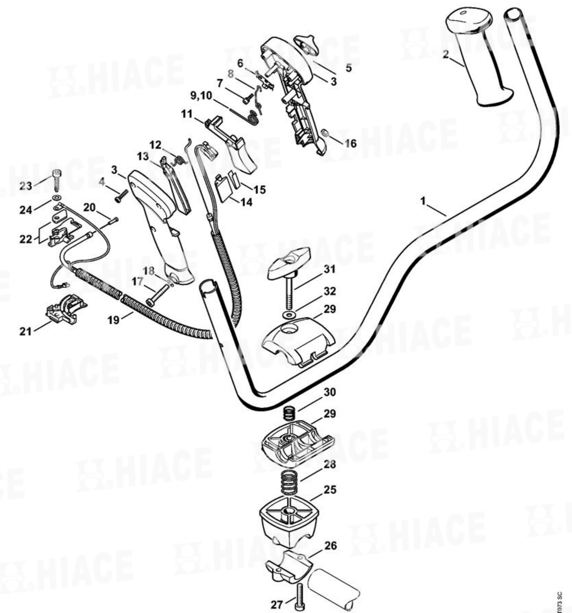
雙手柄 Bike handle
