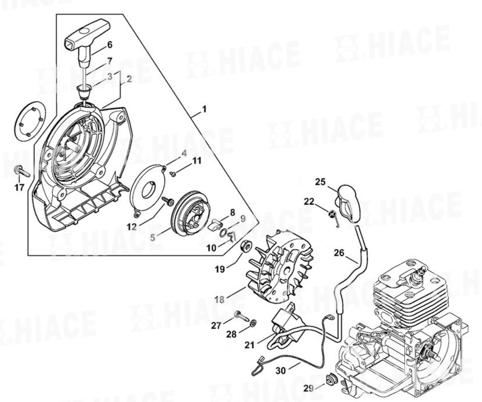
啟動裝置、點火系統 Rewind starter, Ignition system
