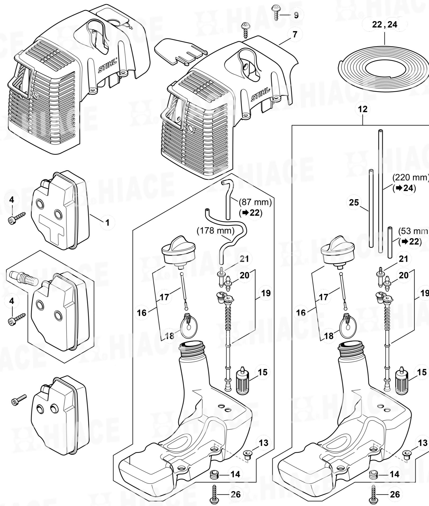
消音器、機罩、燃油箱 Muffler, Shroud, Fuel tank
